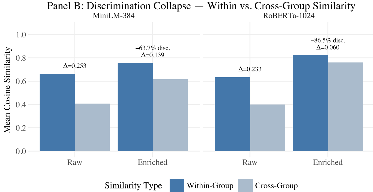
Figure 2: Semantic smearing: group discrimination collapse.
