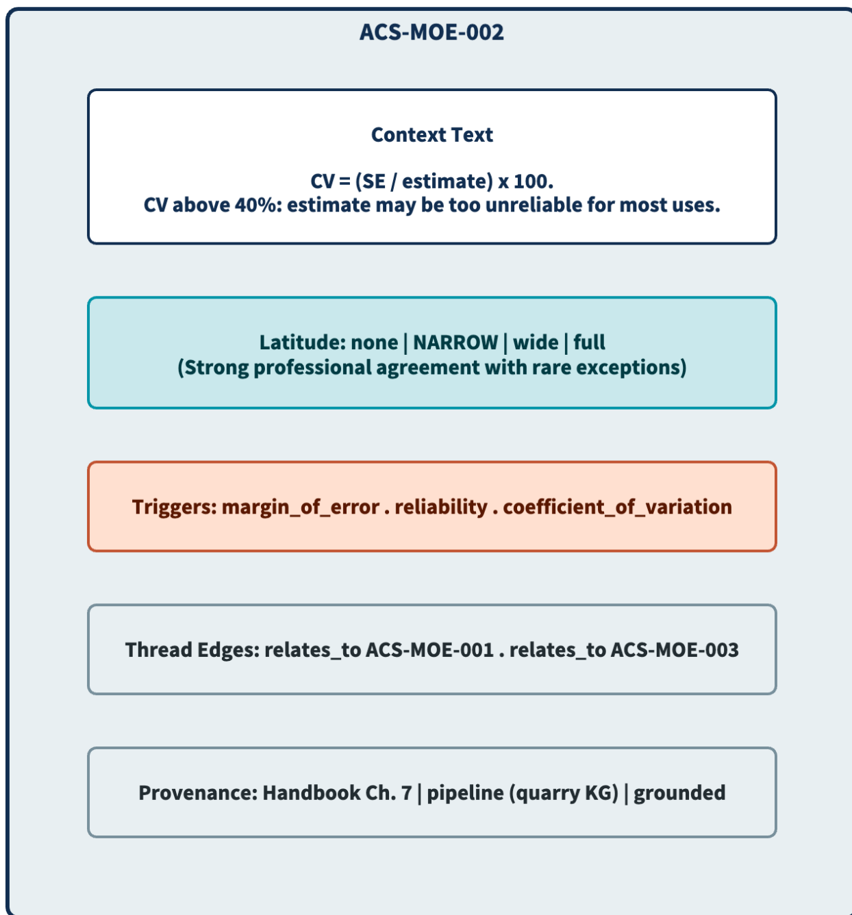
Figure 4: Anatomy of a pragmatic, showing the five structural components using ACS-MOE-002 (coefficient of variation threshold) as an example.
