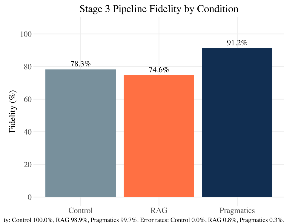
Figure 9: Stage 3 pipeline fidelity by condition. Substantive fidelity (98.9–100.0%) and error rates (0.0–0.8%) annotated in caption.
