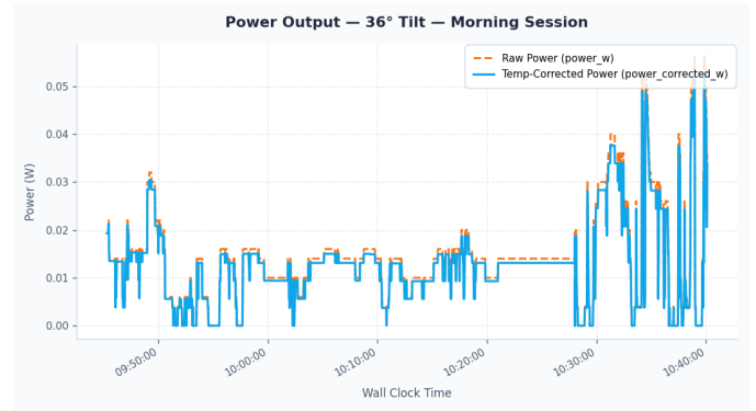
Fig. 9. Power vs. time, 36° morning session.
