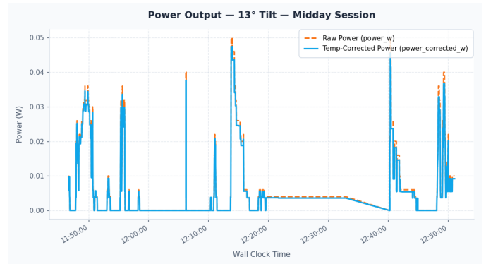
Fig. 8. Power vs. time, 13° midday session.
