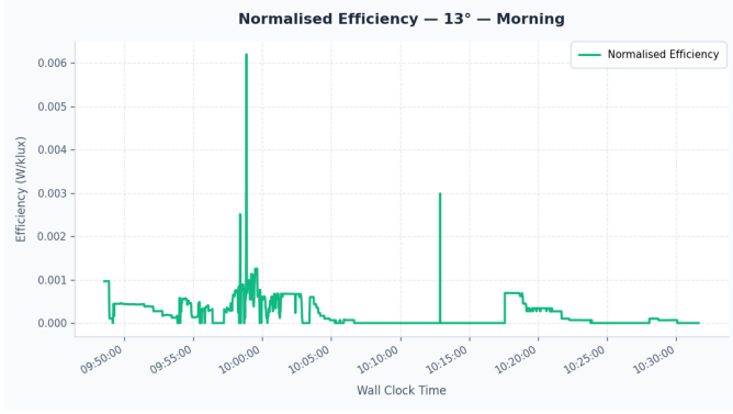
Fig. 11. Normalised efficiency, 13° morning session.
