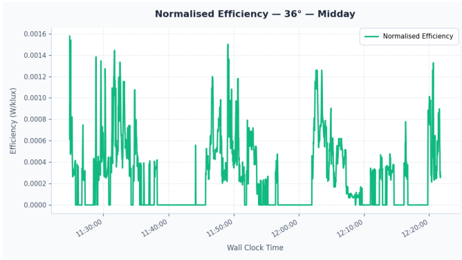
Fig. 12. Normalised efficiency, 36° midday session.
