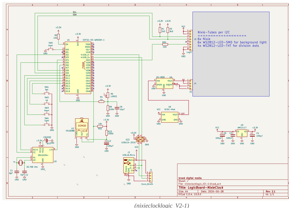
Abb. 1 – Logic Board Rev 2.1 Schaltplan
