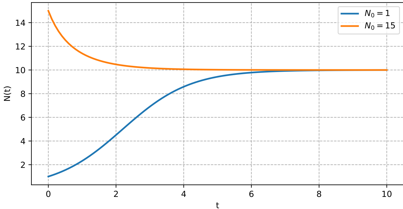
Logistic growth model
