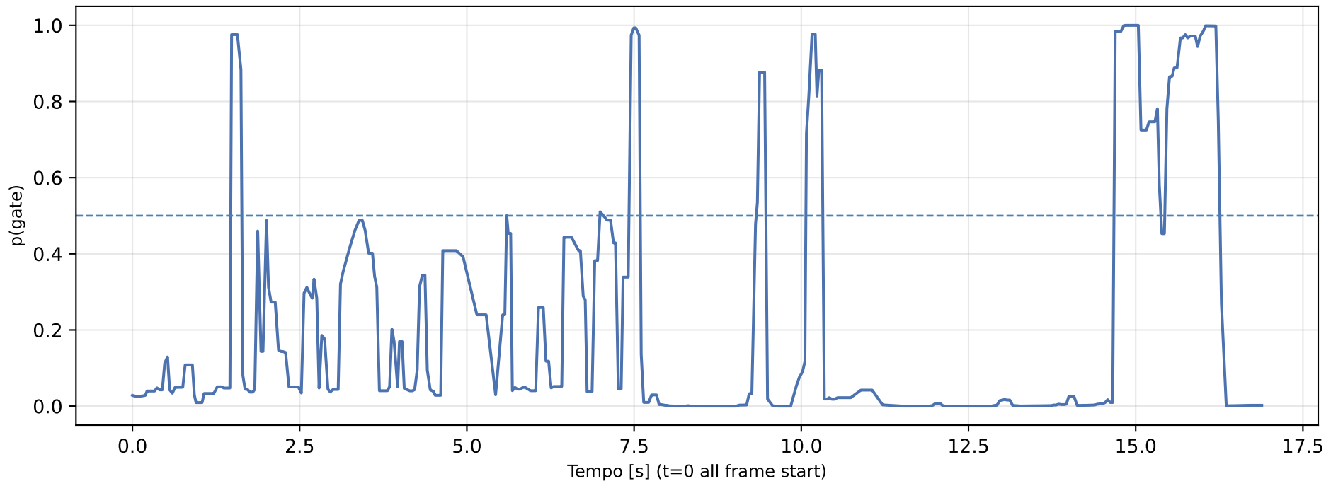
Confidence vs Time | frames 1-392 @ 21.8 fps
