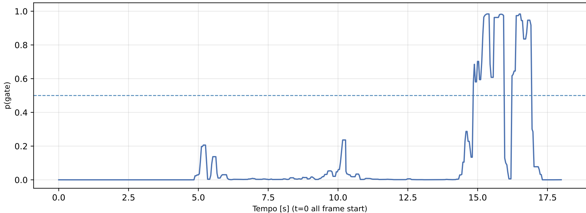
Confidence vs Time | frames 5169-5647 @ 26.6 fps
