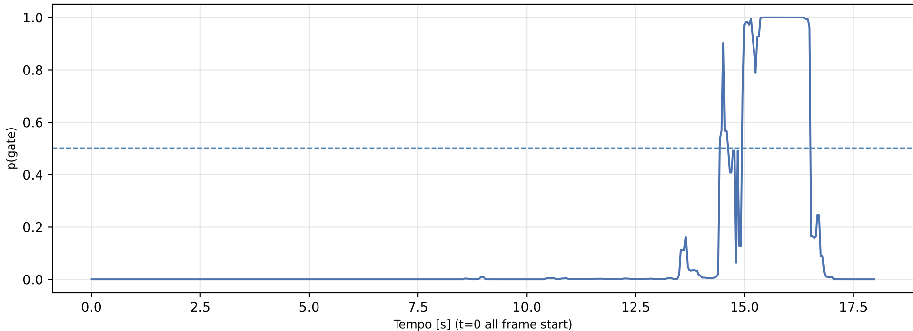
Confidence vs Time | frames 70-551 @ 26.8 fps
