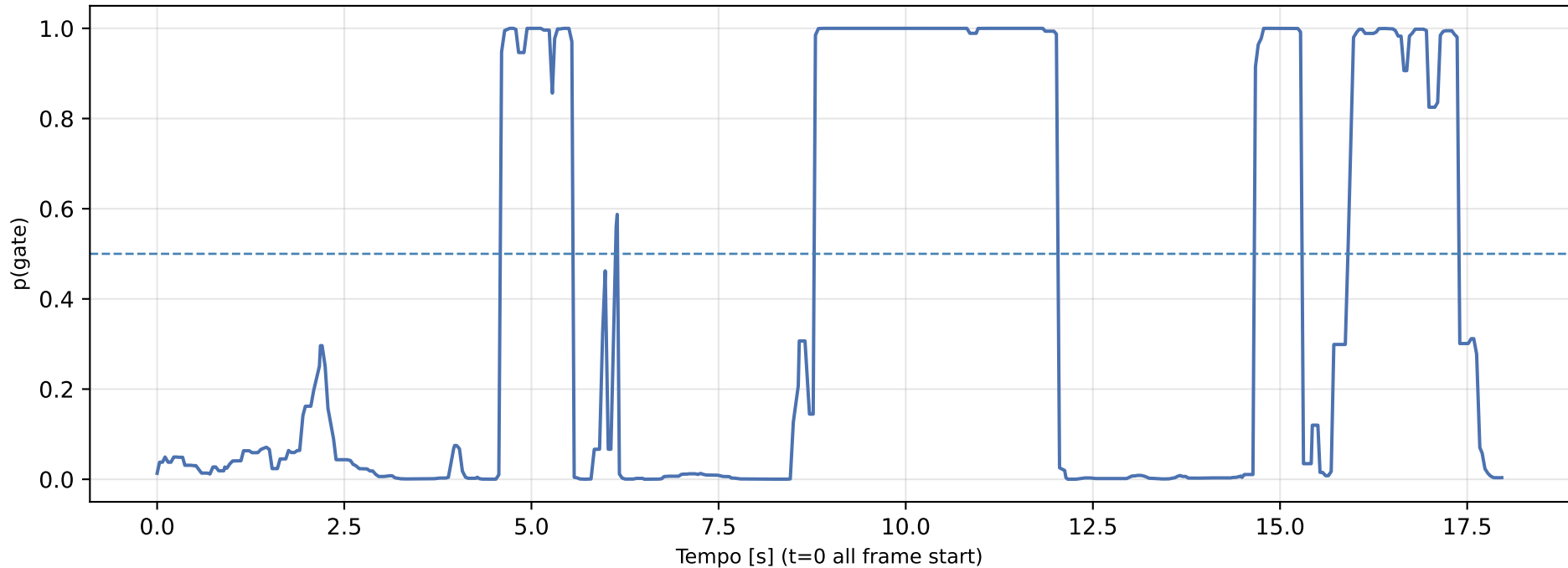
Confidence vs Time | frames 520-999 @ 26.7 fps
