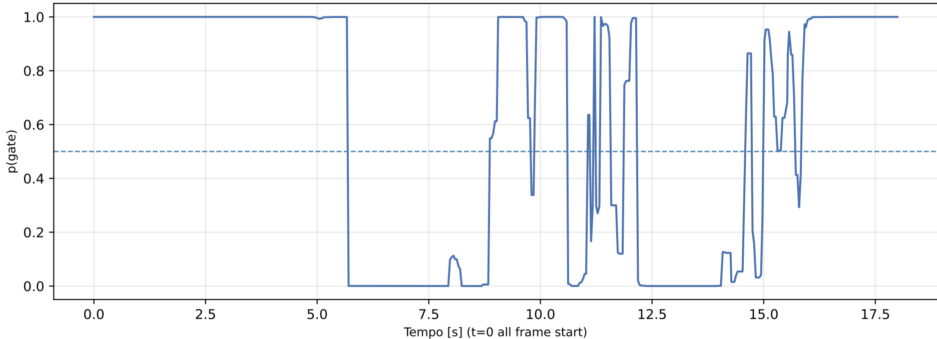
Confidence vs Time | frames 2-486 @ 26.9 fps
