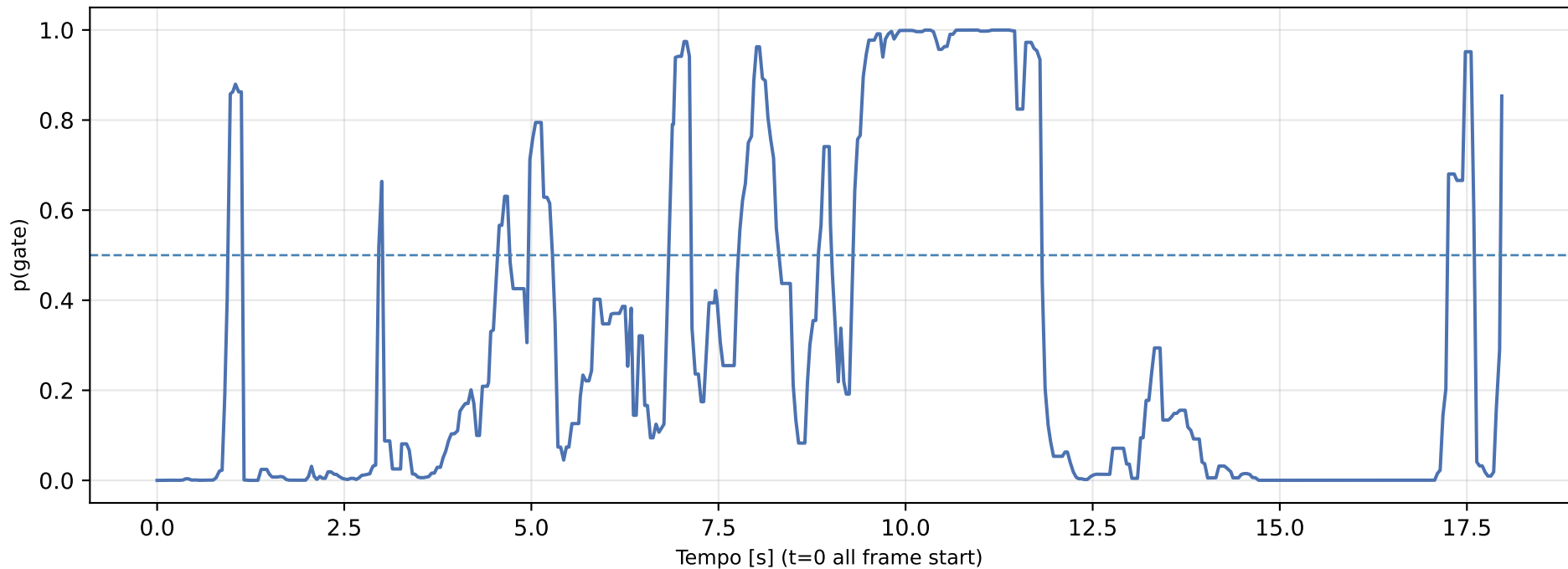
Confidence vs Time | frames 418-896 @ 26.6 fps
