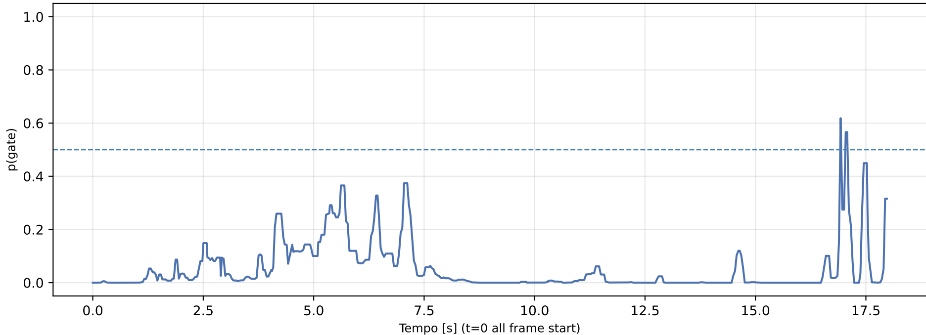
Confidence vs Time | frames 3515-3995 @ 26.7 fps
