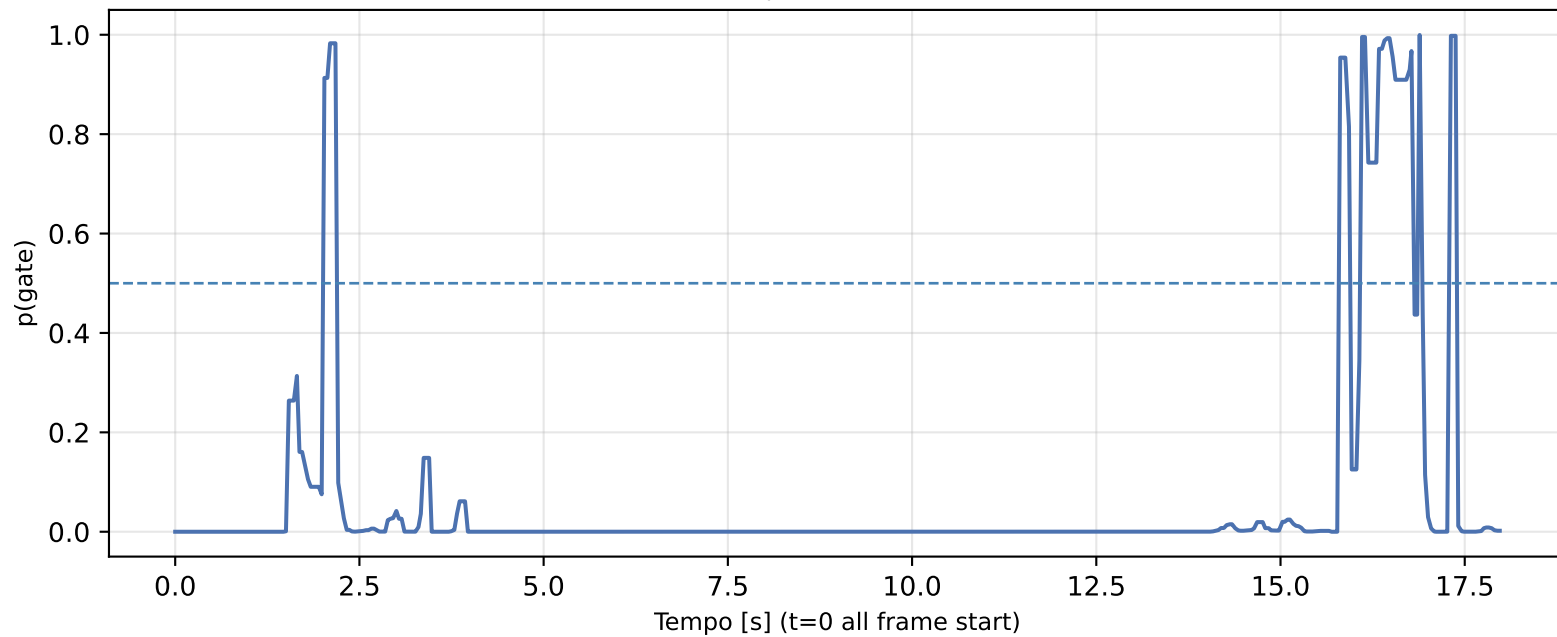
Confidence vs Time | frames 1391-1871 @ 26.7 fps
