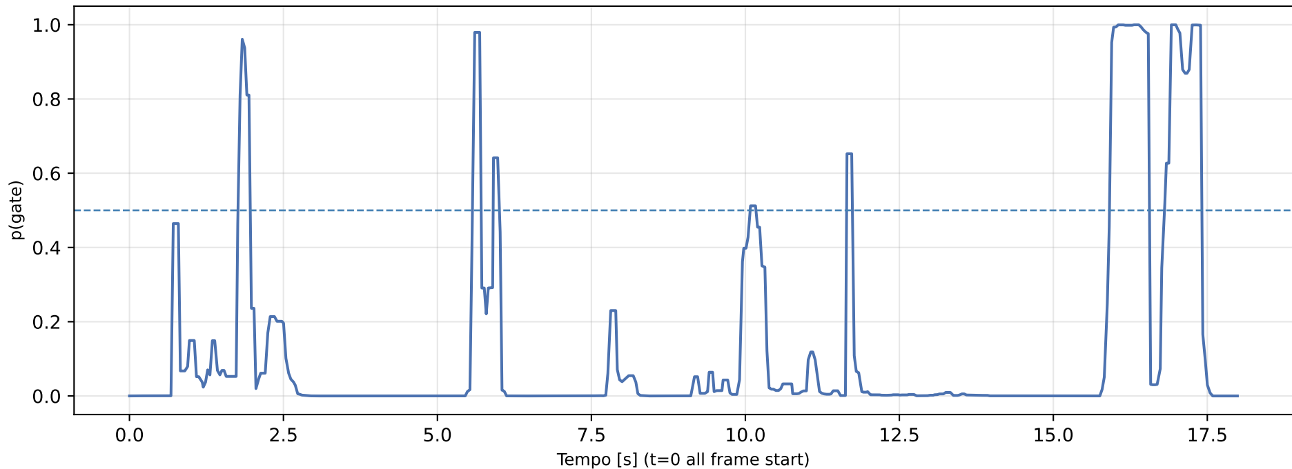
Confidence vs Time | frames 1601-2083 @ 26.8 fps
