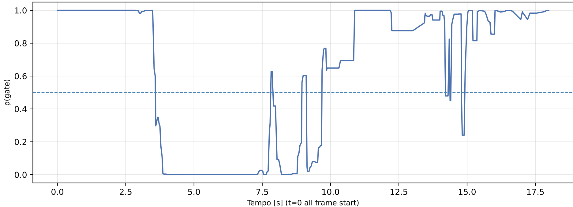
Confidence vs Time | frames 77-466 @ 21.7 fps
