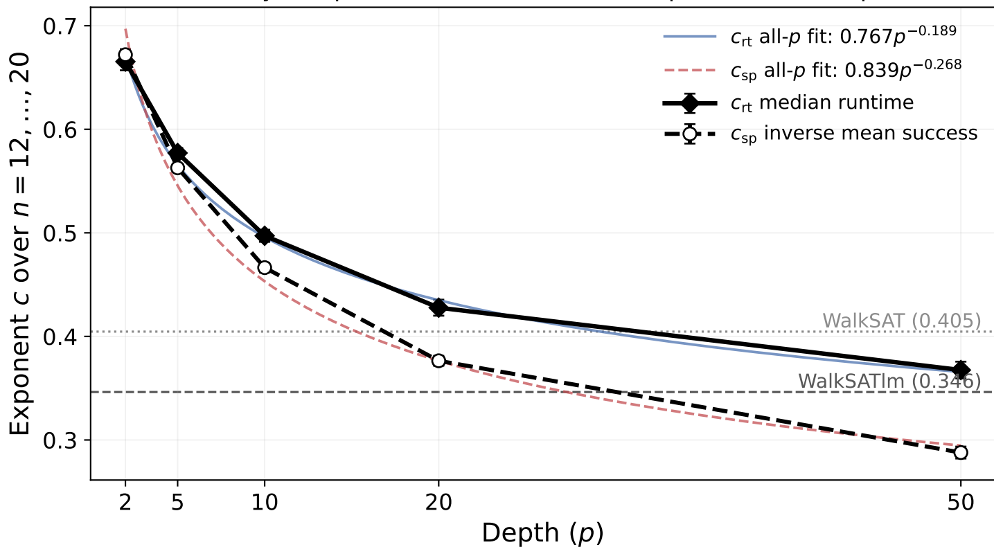
BM24-style exponents: train n=12 , mean- p , N=500-2000 per n
