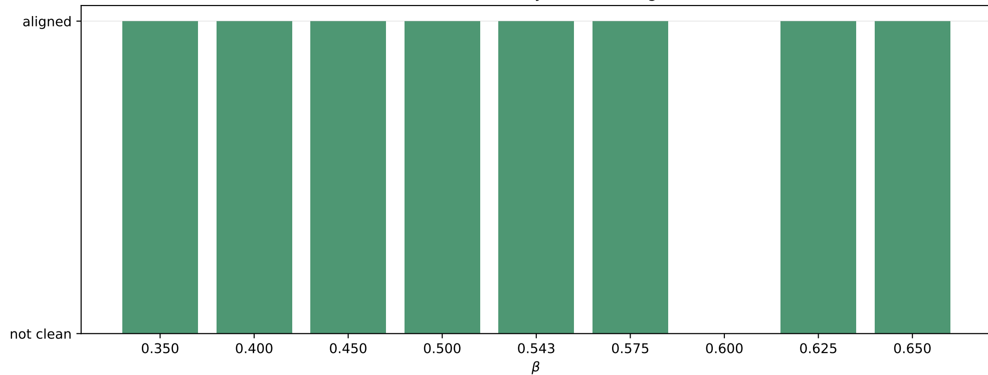
Does the same-branch PL necessary condition align with exact switch?
