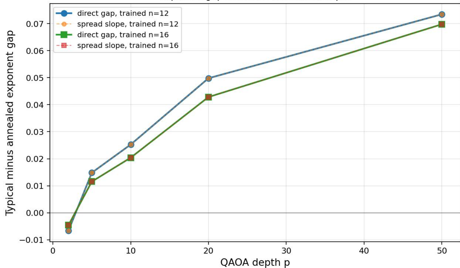
Exponent gap increases with circuit depth
