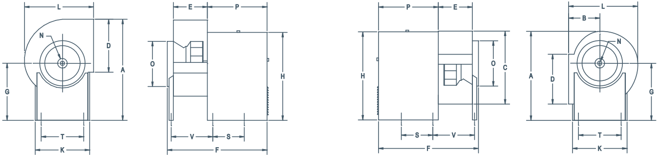
MODELS BI-10 TO BI-27 (STANDARD TOP HORIZONTAL DISCHARGE)
