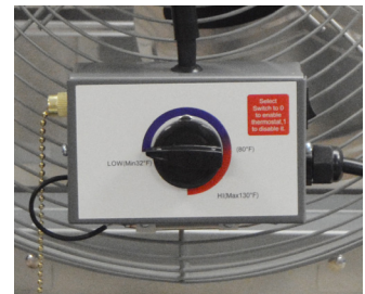
THERMOSTAT CONTROL PANEL
