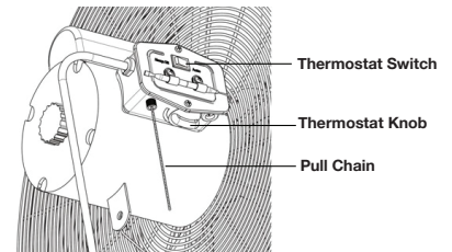
THERMOSTAT CONTROL PANEL
