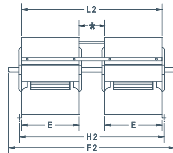
G SERIES TWIN UNITS *SPACING WILL DETERMINE "L2" "H2" AND "F2" DIMENSIONS.
