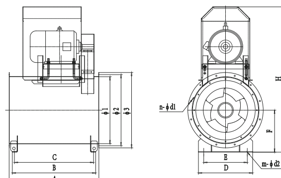
IMF-B560-1250 BASE MOUNTED
