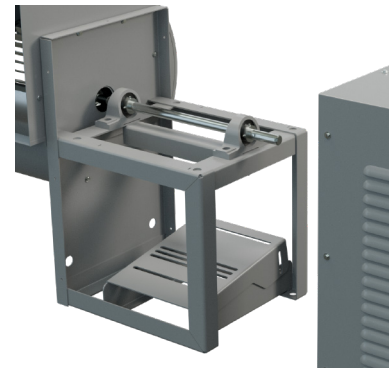
Motor and drive compartment with cover removed showing 3 side motor access and sloping motor base for belt tensioning.
