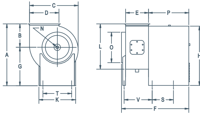
MODELS BI-RM(-HS)-10 TO BI-RM(-HS)-24 (UL 762 LISTED FOR REMOVAL OF COOKING VAPOURS)
