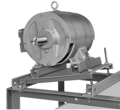
Optional 1 to 15 HP Motor Platform for Models 420, 422 & 425
