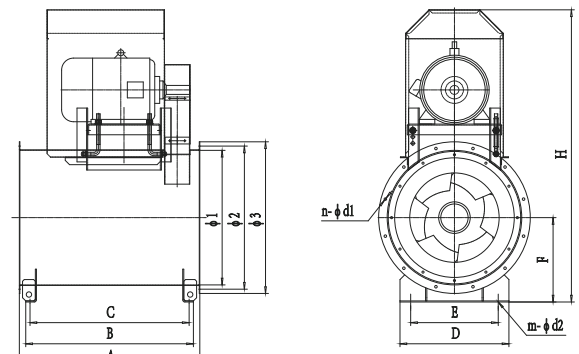
IMF-B560-1250 BASE MOUNTED
