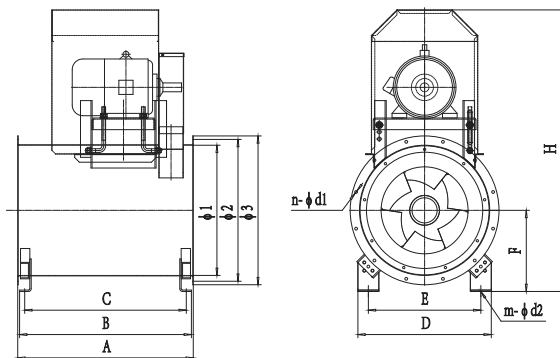
IMF-B400-500 BASE MOUNTED
