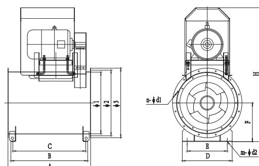
IMF-B560-1250 BASE MOUNTED
