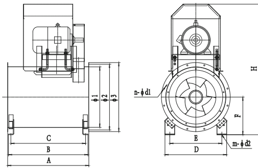
IMF-B400-500 BASE MOUNTED
