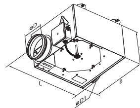
FIGURE 1 - Inline Dryer Booster Fan
