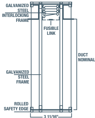
TYPICAL VERTICAL DAMPER
