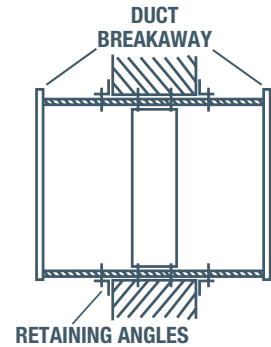
SUGGESTED INSTALLATION
