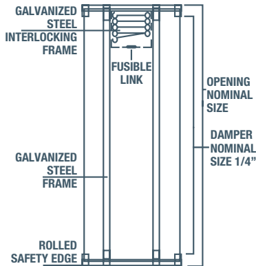
TYPICAL VERTICAL DAMPER
