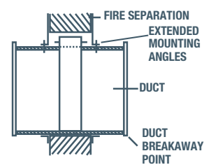
ALTERNATE INSTALLATION
