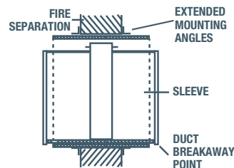
SUGGESTED INSTALLATION
