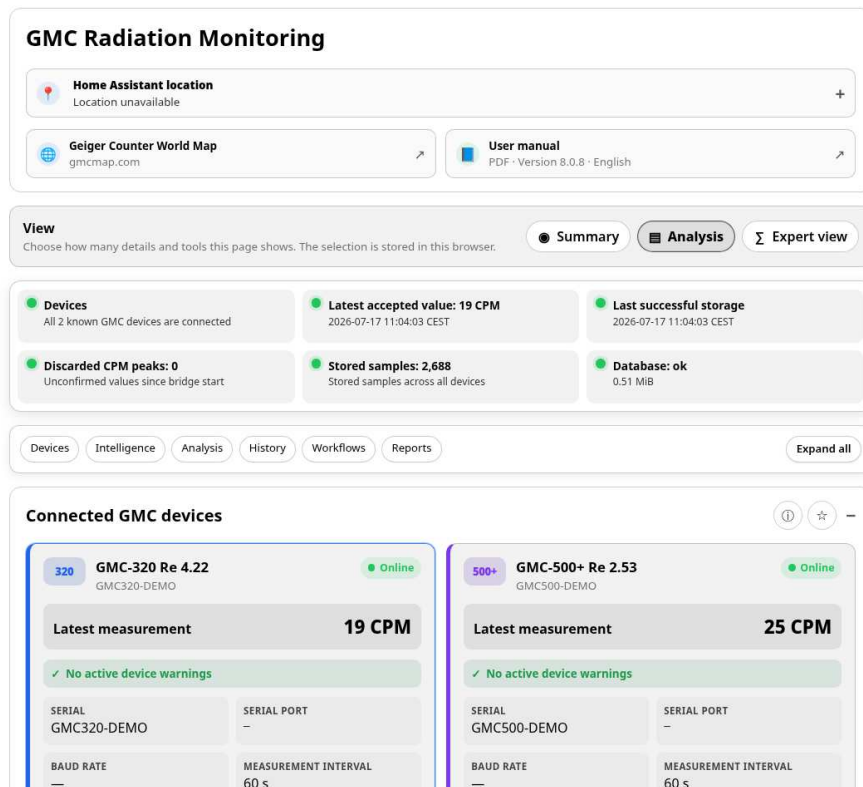
4. Dashboard overview
