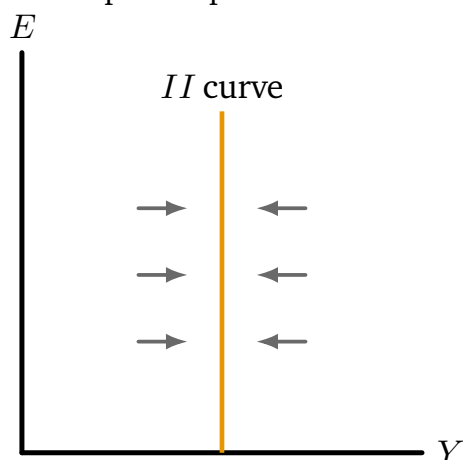
Figure 1.2: II dynamics.
