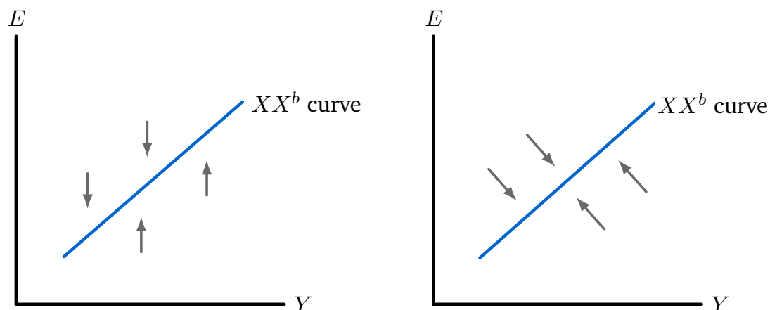
Figure 1.4: XX dynamics.
