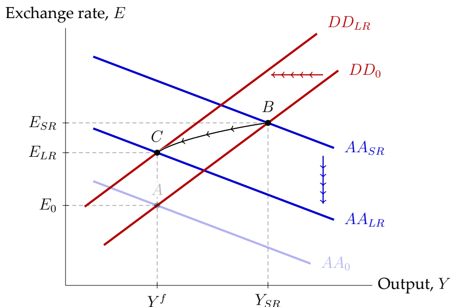
Figure 2: Permanent reduction in money demand: transition from the short run to the long run.
