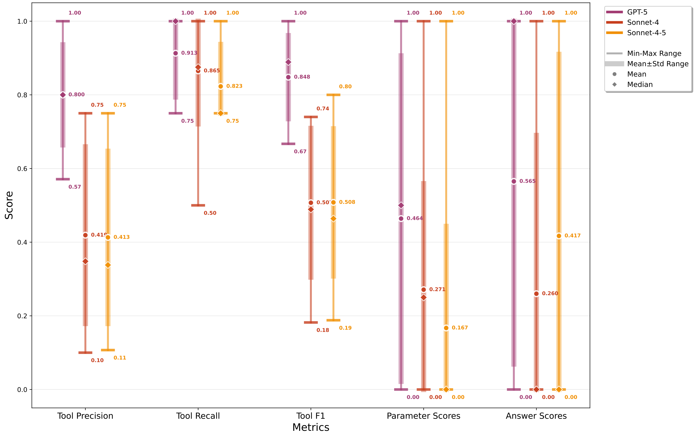
GDS agent on graph-agent-bench-got-v1 dataset with different LLMs. No tool descriptions.
