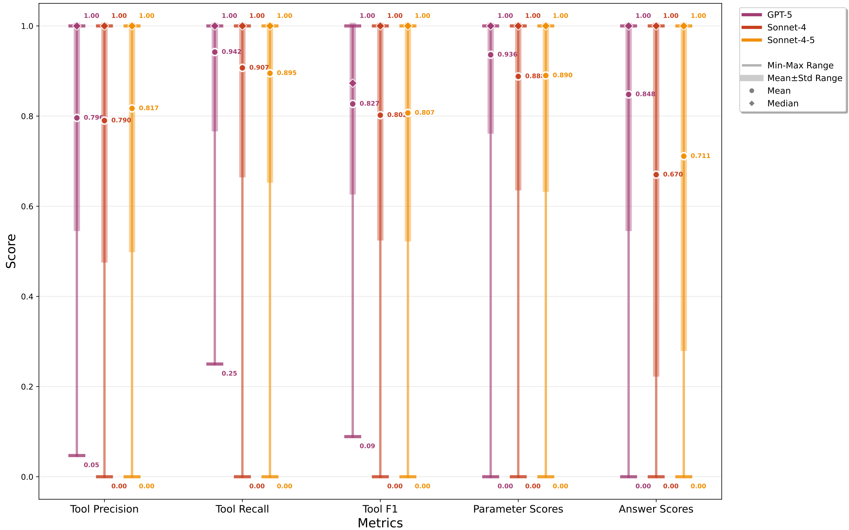
GDS agent on graph-agent-bench-ln-v1 dataset with different LLMs. No tool descriptions.
