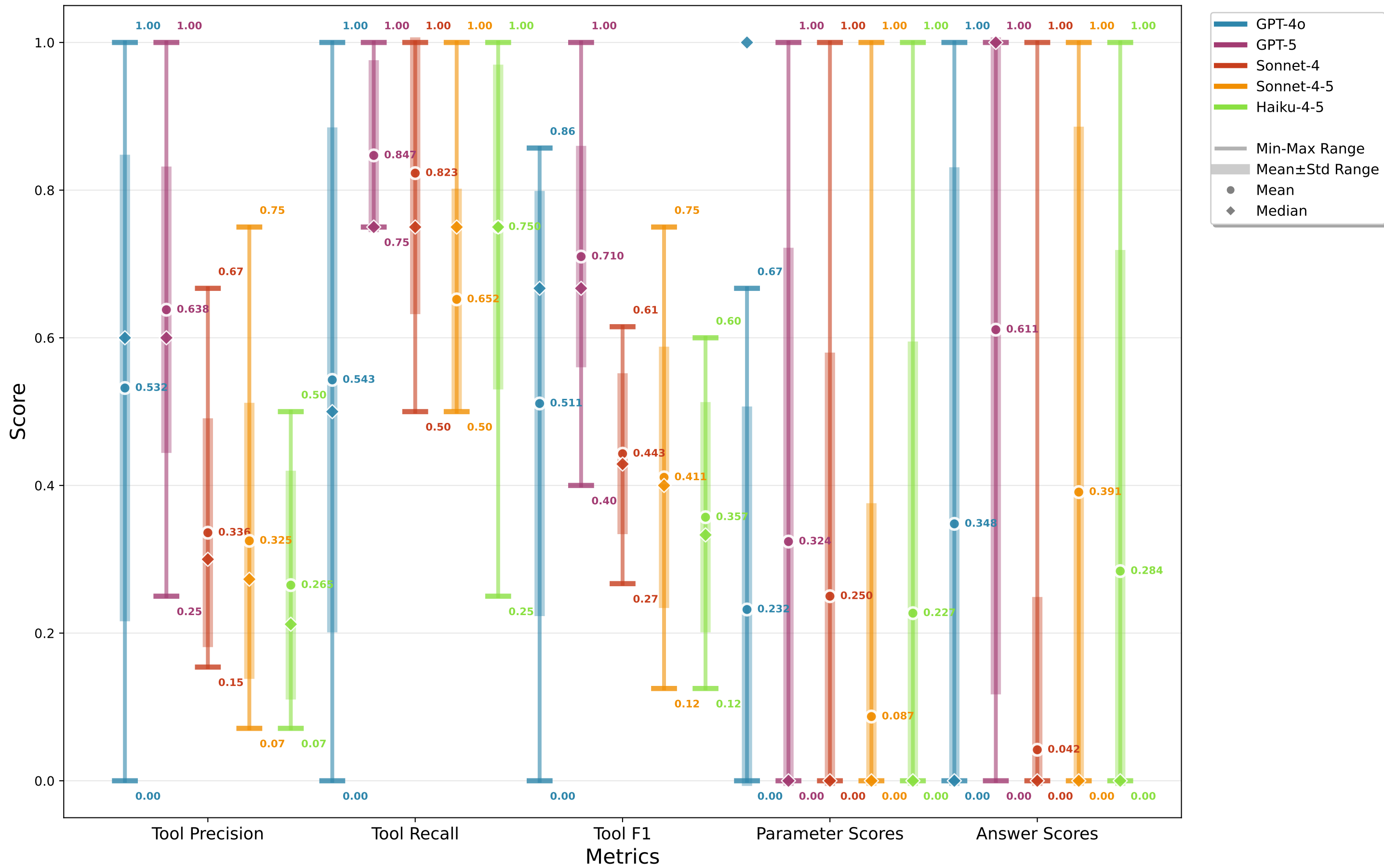
GDS agent on graph-agent-bench-got-v1 dataset with different LLMs. No tool & No param descriptions.
