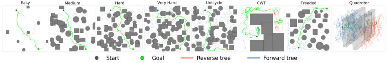
Fig. 3: Final BBoE solutions showing unicycle environments across four difficulty tiers (seed 15795) and four different dynamical systems. The forward tree (blue) traces the reverse tree (red) into the goal region. The solution path (green) consists of forward-tree edges.
