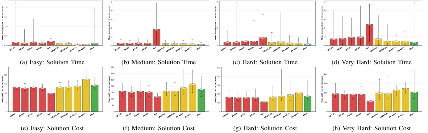
Fig. 6: Unicycle planner evaluation across 40 environments (10 per difficulty tier, 50 seeds each). Top row: Mean initial solution time on successes per difficulty. Bottom row: Mean solution cost on successes per difficulty.
