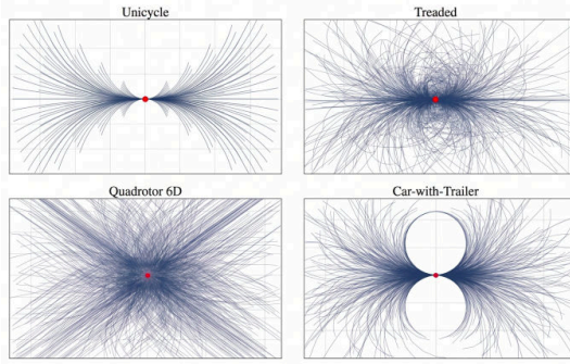
Fig. 4: The 2-dimensional projection of a subset of the edges generated for each system. Every edge starts at the origin of the XY plane. The unicycle edges are essentially the maneuver libraries used in the GBRRT paper.
