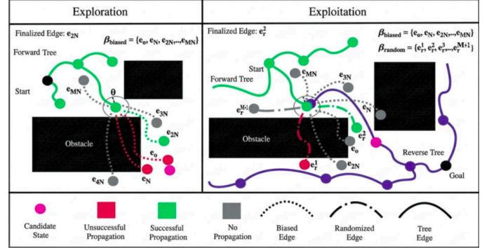
Fig. 1: The functionality of BBoE encompasses two phases, exploration and exploitation. During exploration, the forward tree primarily uses the biased edges ( \beta_{biased} ) to expand towards the candidate state, while the reverse tree relies on propagating random edges backward in time. During exploitation, either the biased edges or the randomized edges ( \beta_{random} ) are used while allowing the forward tree to accurately trace the reverse tree towards the goal.
