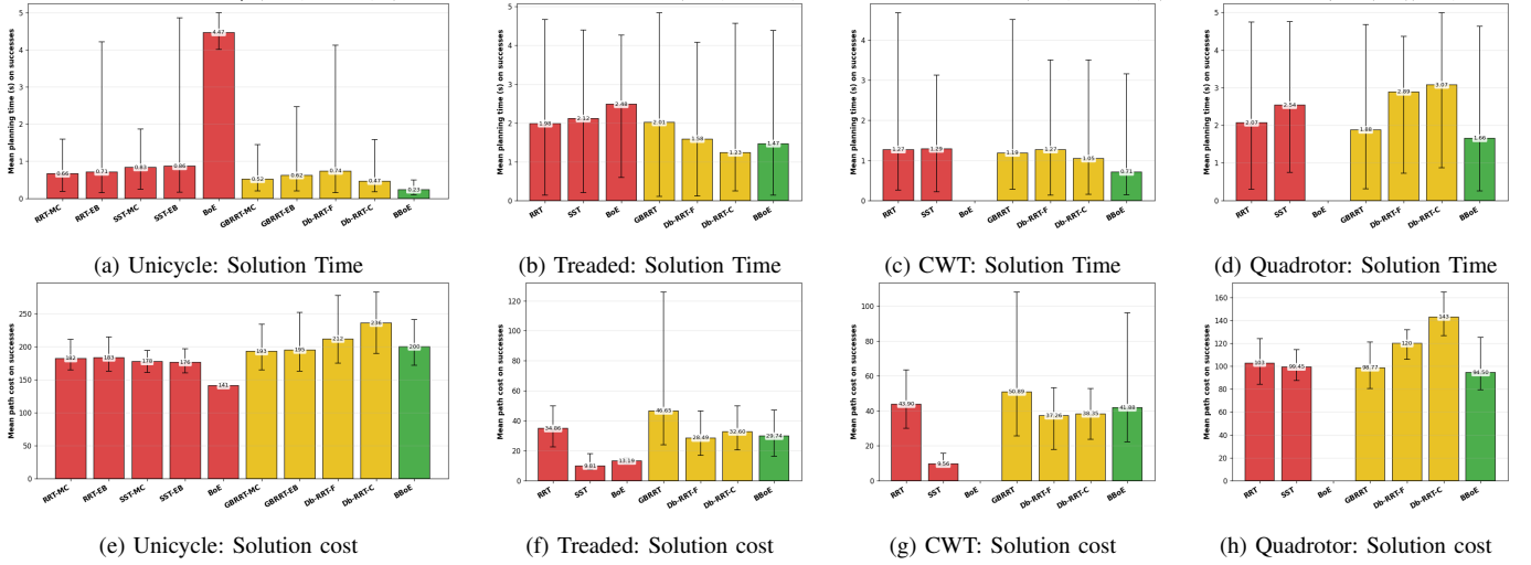
Fig. 5: Cross-system planner evaluation on the unicycle, treaded vehicle, car-with-trailer (CWT), and quadrotor (50 seeds each). Top row: mean initial solution time on successes per system. Bottom row: mean solution cost on successes per system. BBoE achieves the lowest planning time on three of four systems and \geq 96\% success on every system.
