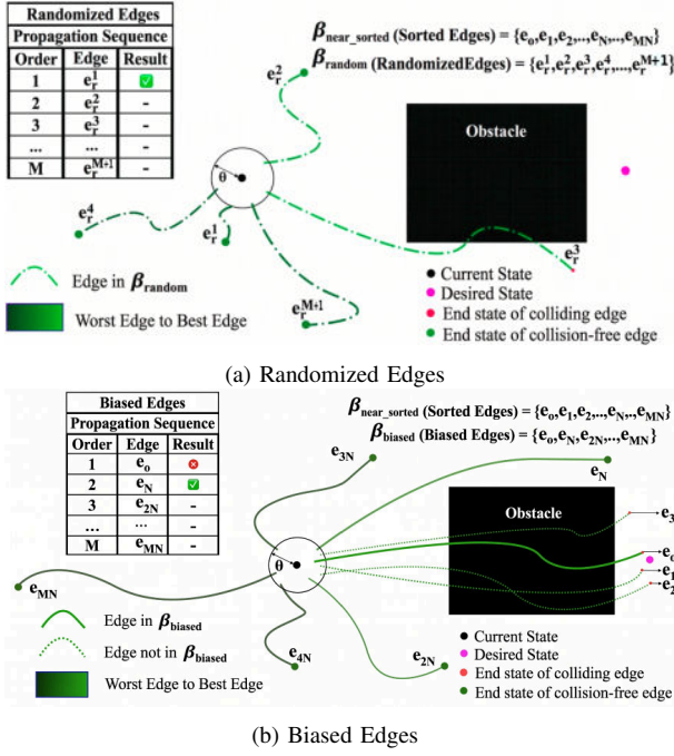
Fig. 2: Given the robot’s current state, we gather all edges initiating within a radius of \theta from it and store them in \beta_{\text{near\_sorted}} . From this set, we extract relevant edges and store them in sets \beta_{\text{random}} (a) and \beta_{\text{biased}} (b). We show the exact order of edge propagation in each scenario with the result.
