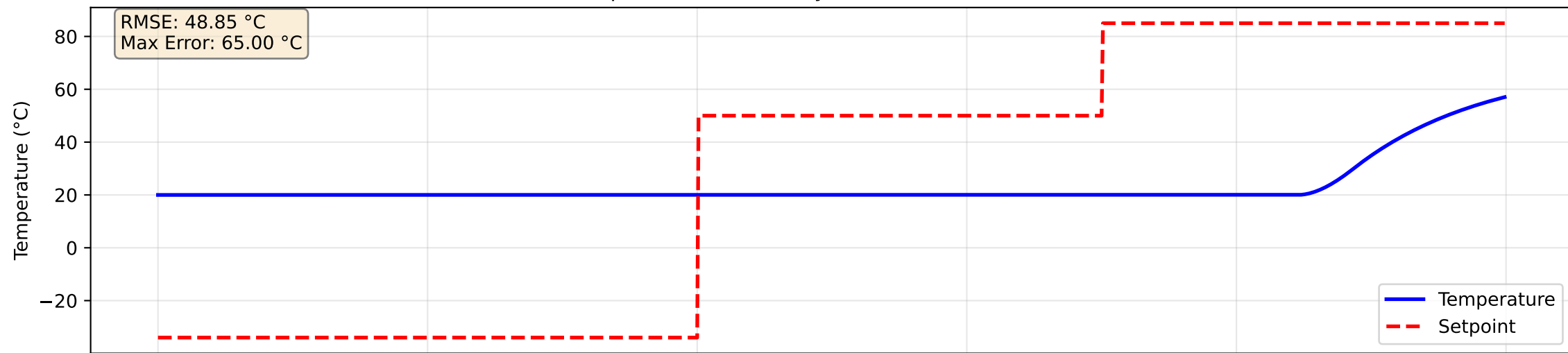
Temperature Control System with PID Controller
