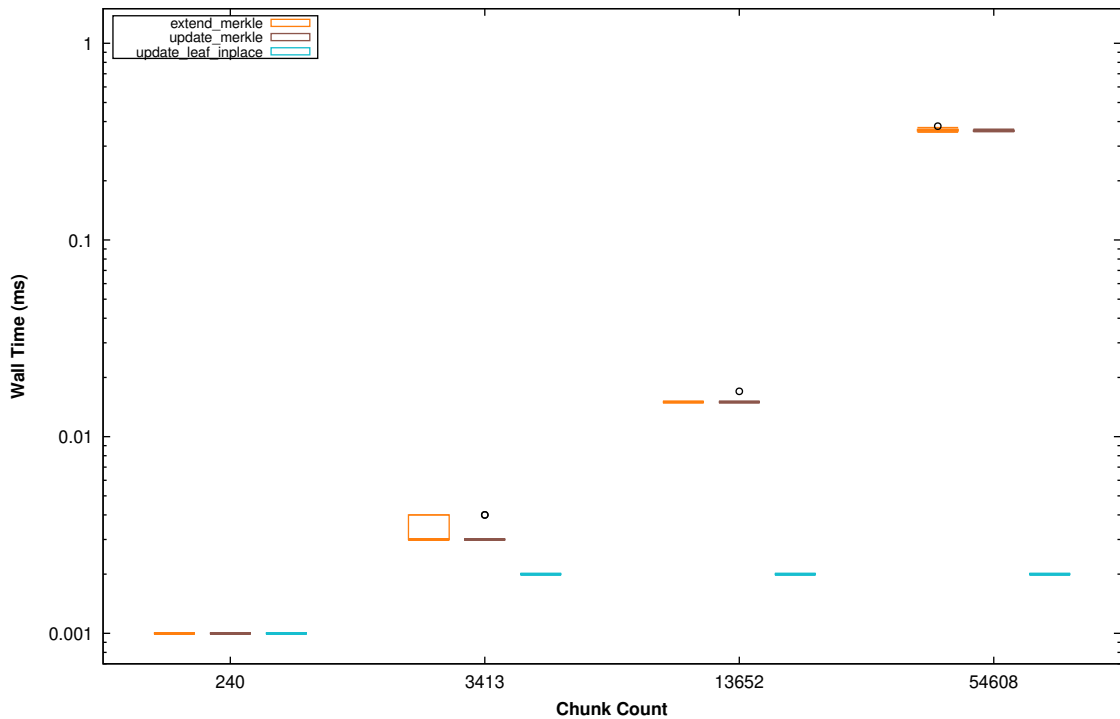
extend_merkle / update_merkle / update_leaf_inplace: per-cell distribution (30 trials)
