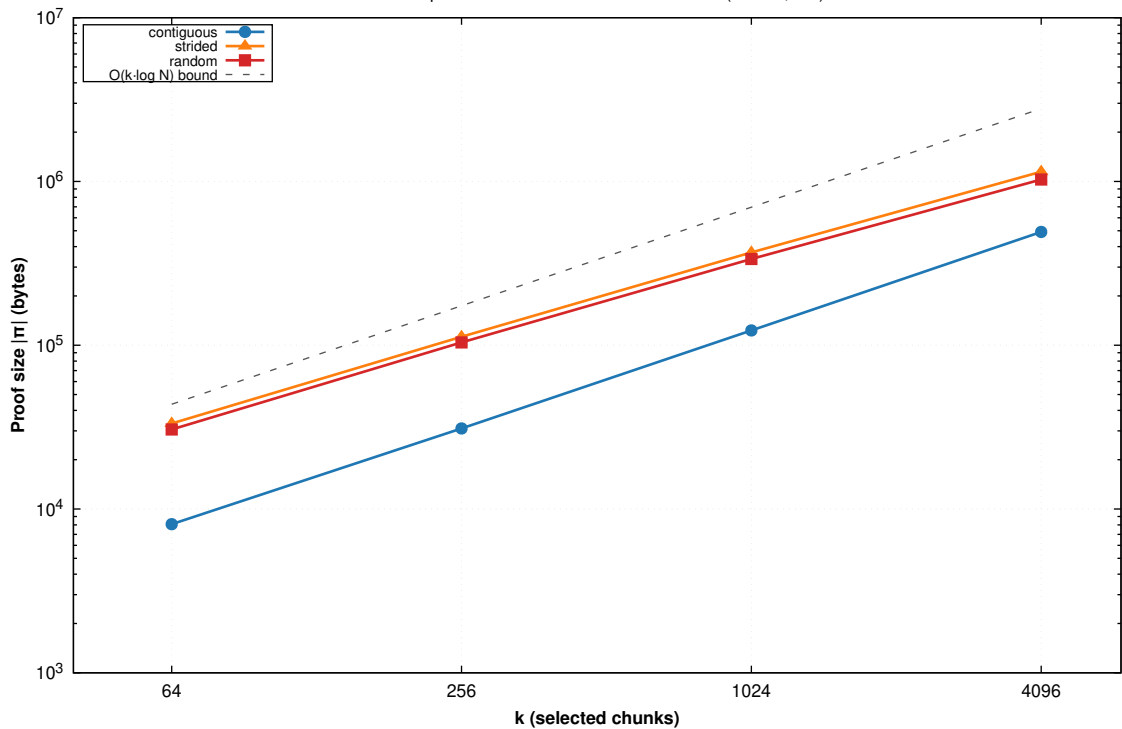
Subset-proof size vs. selected-chunk count k ( N = 65,536 )
