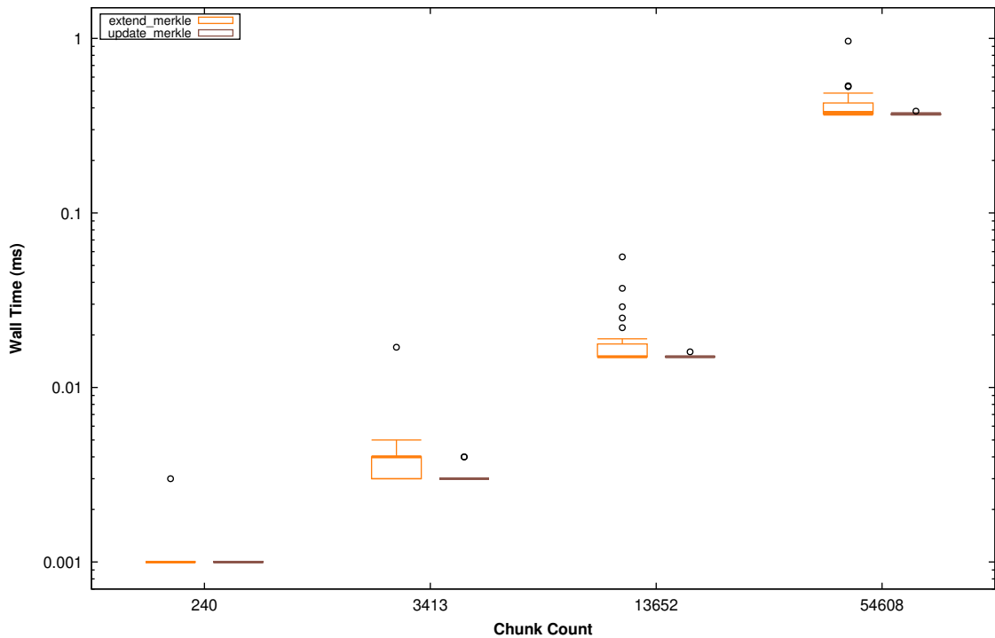
extend_merkle / update_merkle: per-cell distribution (30 trials)
