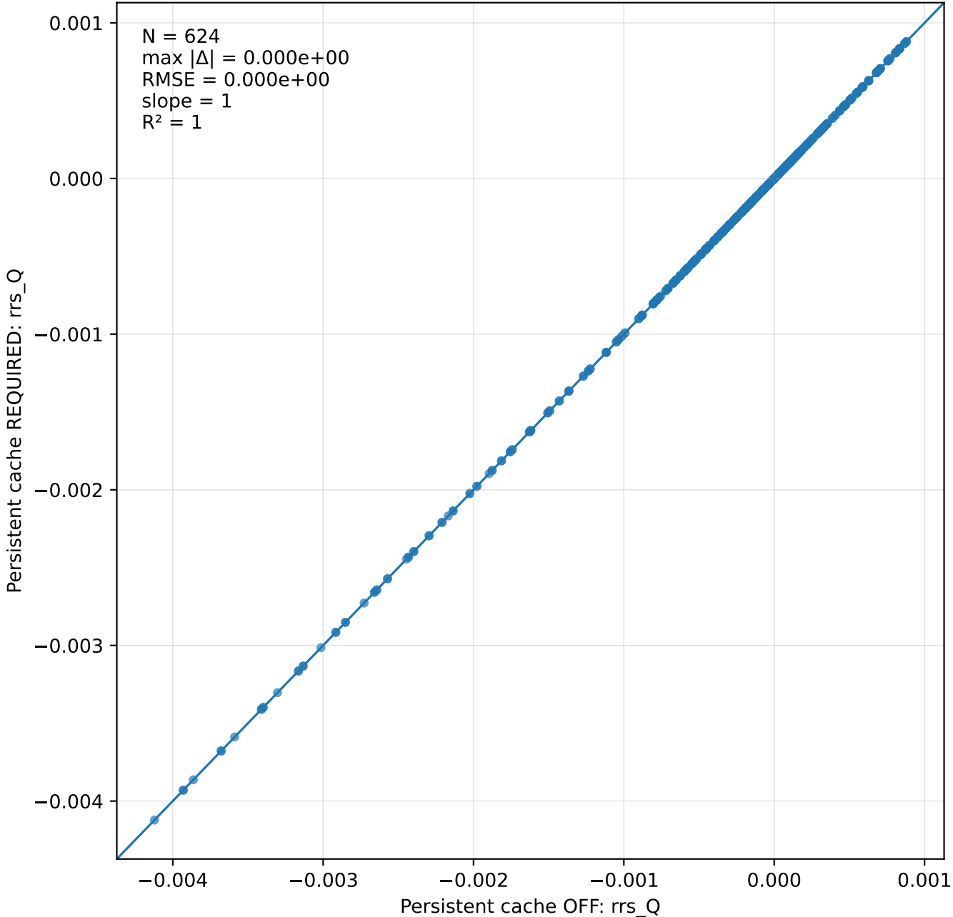
OCRT persistent Cox-Munk/interface cache regression — rrs_Q
