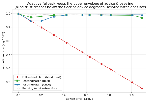
Figure 6.1: The robustness envelope: blind FollowPrediction crashes below the advice-free floor as advice error grows; TestAndMatch stays on the upper envelope.
