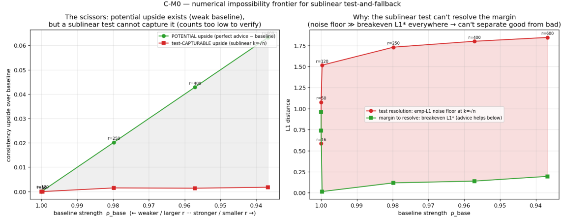
Fig. 7. The budget–stakes scissors: as the baseline weakens (left), the potential upside of perfect advice grows, while the upside a feasible test can safely capture stays pinned near zero — the empirical test’s resolution sits far above the break-even margin wherever the upside exists.
