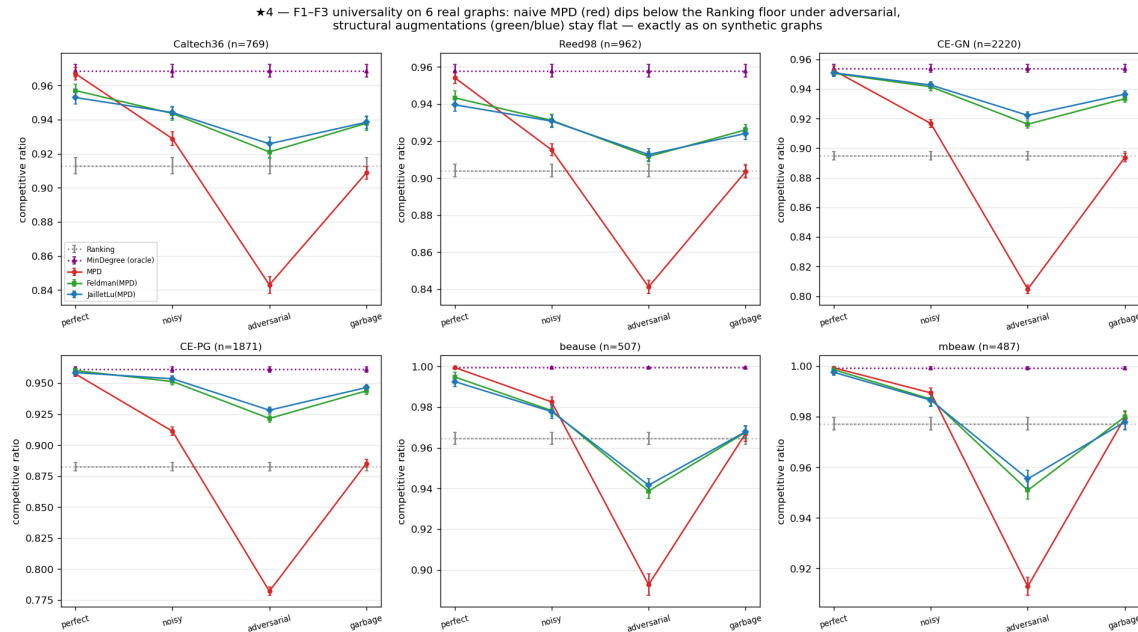
Fig. 6. The six real-world graphs: ungarded following falls below the advice-free floor on every graph, and the augmentation restores safety — the benchmark’s findings are universal, not generator artifacts.
