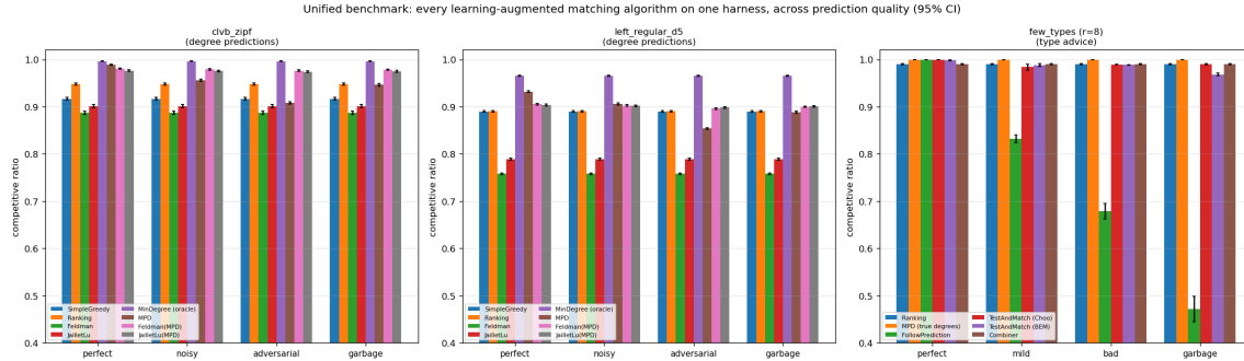
Fig. 1. The unified benchmark (Table 1) as grouped bars: competitive ratio by algorithm and advice quality, one group per panel; the advice-free floor and oracle ceiling bracket every bar.
