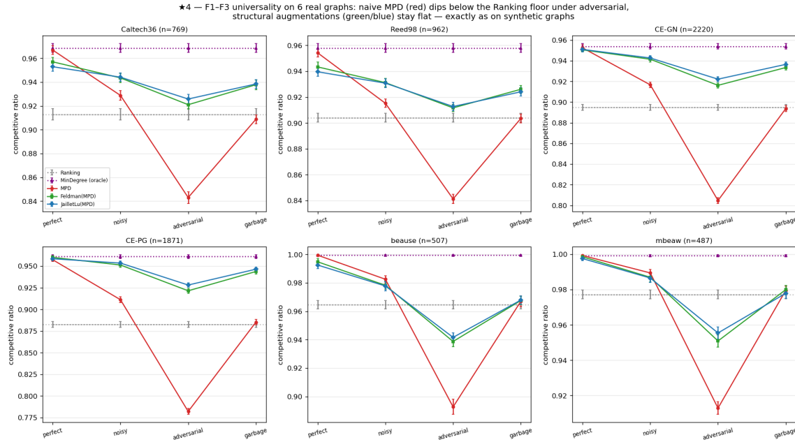
Fig. 8. The six real-world graphs: ungarded following falls below the advice-free floor on every graph, and the augmentation restores safety — the benchmark’s findings are universal, not generator artifacts.
