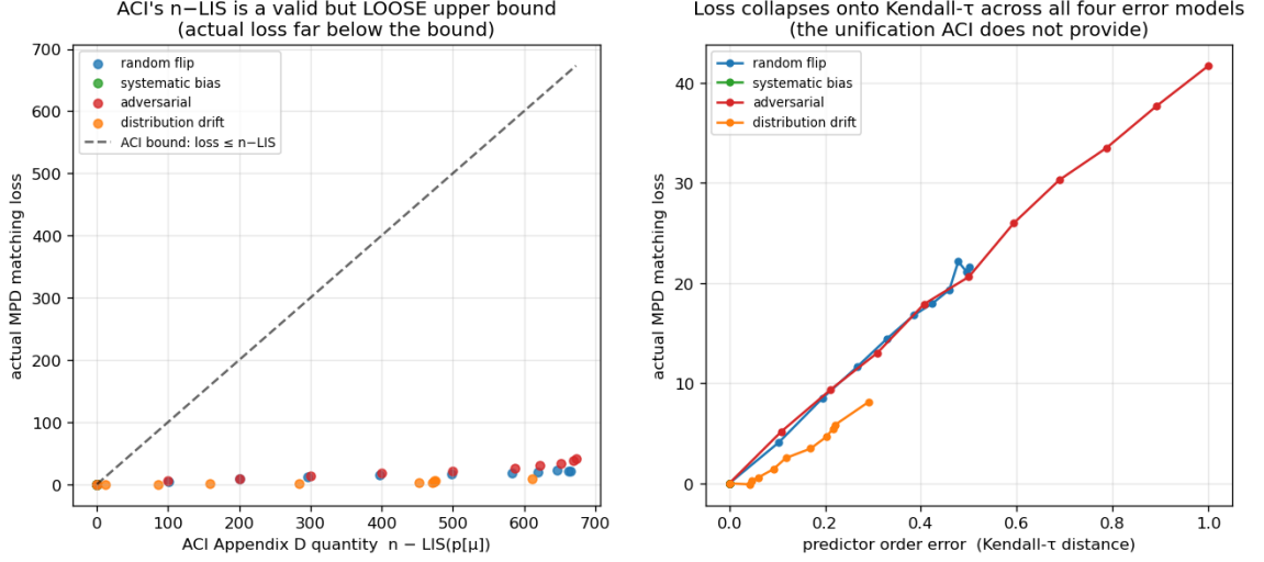
Fig. 2. Order error, not magnitude, governs MPD's loss: (a) realized loss sits far below the n - \text{LIS} bound at every point; (b) the four error models collapse onto the Kendall- \tau axis.
