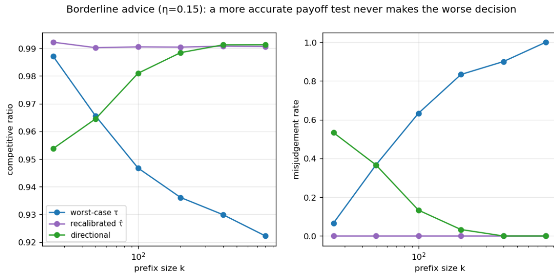
Fig. 6. Borderline advice ( \eta = 0.15 ): as the prefix grows, the worst-case threshold’s misjudgement rises to 1.0 while the payoff rule’s falls to 0.0 — more data helps exactly when the statistic is the decision-relevant one.
