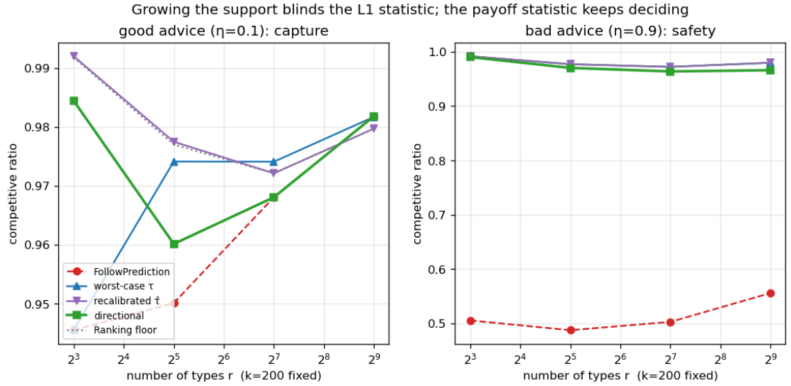
Fig. 10. The blindness curve on the benchmark generator: at fixed true \ell_1 \approx 0.11 and k = 200 , the plug-in \hat{\ell}_1 inflates with the support size while the payoff rule keeps deciding at both good (left) and bad (right) advice.
