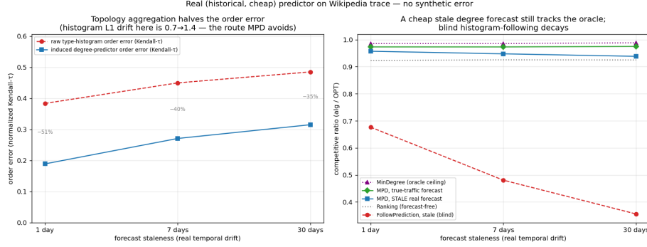
Fig. 7. A cheap historical-count predictor on the Wikipedia trace: near-oracle ratio at every staleness level, never below the advice-free floor.
