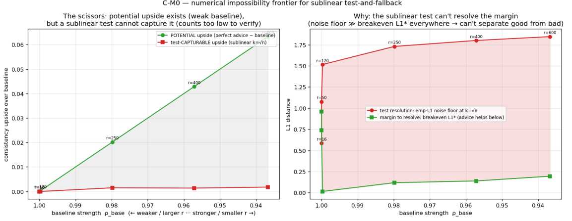
Fig. 9. The budget–stakes scissors: as the baseline weakens (left), the potential upside of perfect advice grows, while the upside a feasible test can safely capture stays pinned near zero — the empirical test’s resolution sits far above the break-even margin wherever the upside exists.
