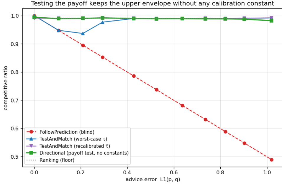
Fig. 5. The envelope sweep with the payoff rule added: the worst-case threshold follows the crash at mildly bad advice, the recalibrated threshold never captures at perfect advice, and the constant-free payoff rule tracks the upper envelope within the resolution the budget-stakes law allows.
