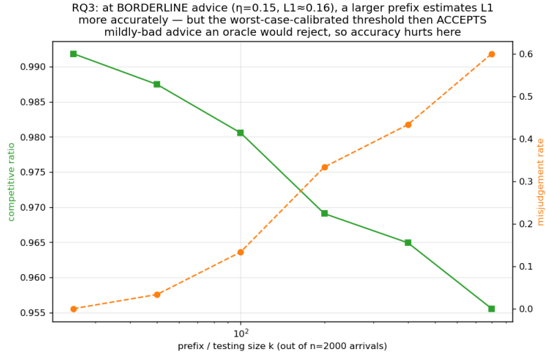
Fig. 4. Testing cost at borderline advice: under the worst-case-calibrated threshold, a larger and more accurate prefix test makes the worse decision.
