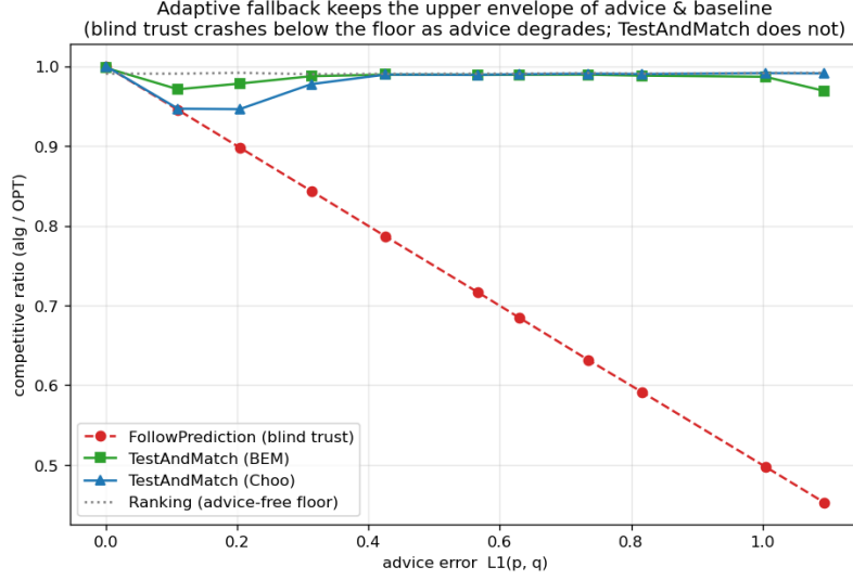
Fig. 3. The robustness envelope: blind FollowPrediction crashes below the advice-free floor as advice error grows; TestAndMatch stays on the upper envelope.
