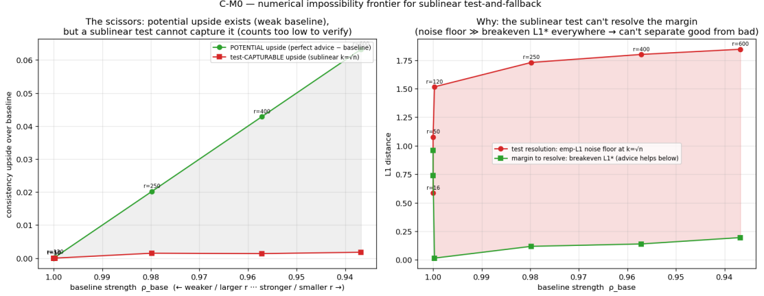
Figure 9.1.: The impossibility, numerically (the “scissors”). Left: the potential upside grows as the baseline weakens, but the upside a sublinear test can safely capture stays near zero. Right: the test’s empirical- \ell_1 resolution sits far above the break-even margin wherever an upside exists.
