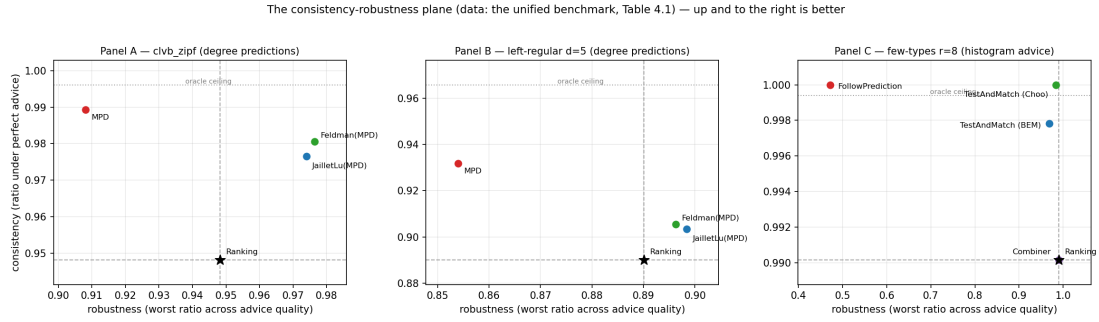
Figure 4.2.: The consistency–robustness plane, one point per algorithm (consistency = ratio under perfect advice; robustness = worst ratio across advice quality; the data of Table 4.1). Dashed lines mark the advice-free floor, dotted the oracle ceiling. Naive followers (MPD, FollowPrediction) buy consistency with robustness; the structural augmentations give up little of either; TestAndMatch sits nearest the ideal top-right corner; the combiner stays pinned at the floor point.
