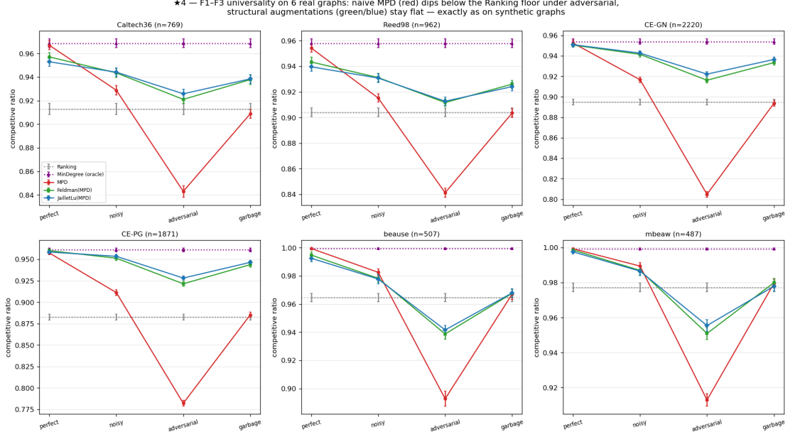
Figure 7.2.: F1–F3 on six real graphs. Naive MPD (red) dips below the Ranking floor under adversarial predictions on every graph; the structural augmentations (green/blue) stay flat — as on synthetic graphs.
