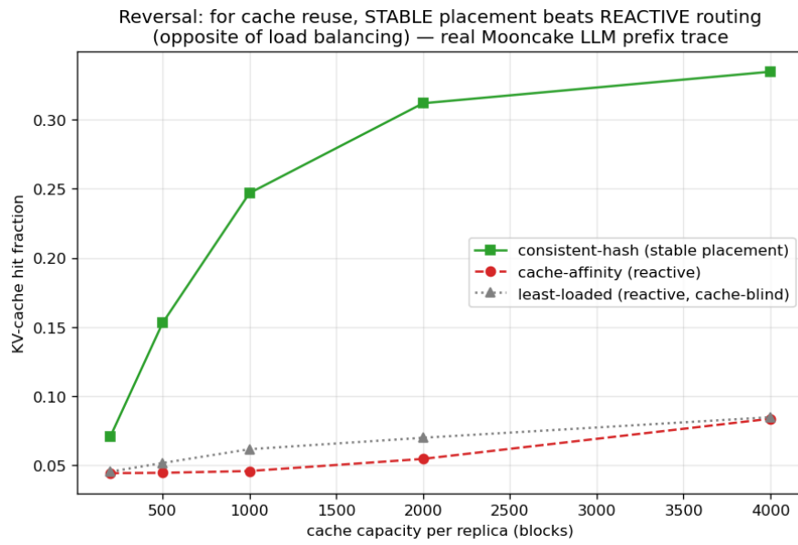
Figure 10.3.: The cache-affinity reversal (real Mooncake prefix trace): for KV-cache reuse, a stable consistent-hash placement beats reactive routing — the opposite of the load-balancing case — because cache locality rewards persistence.
