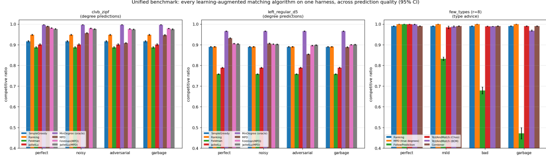
Figure 4.1.: The unified benchmark: competitive ratio (mean, 95% CI) versus prediction quality, for the three panels. Naive followers (MPD under adversarial, FollowPrediction) dip below the advice-free floor; the robust algorithms do not.
