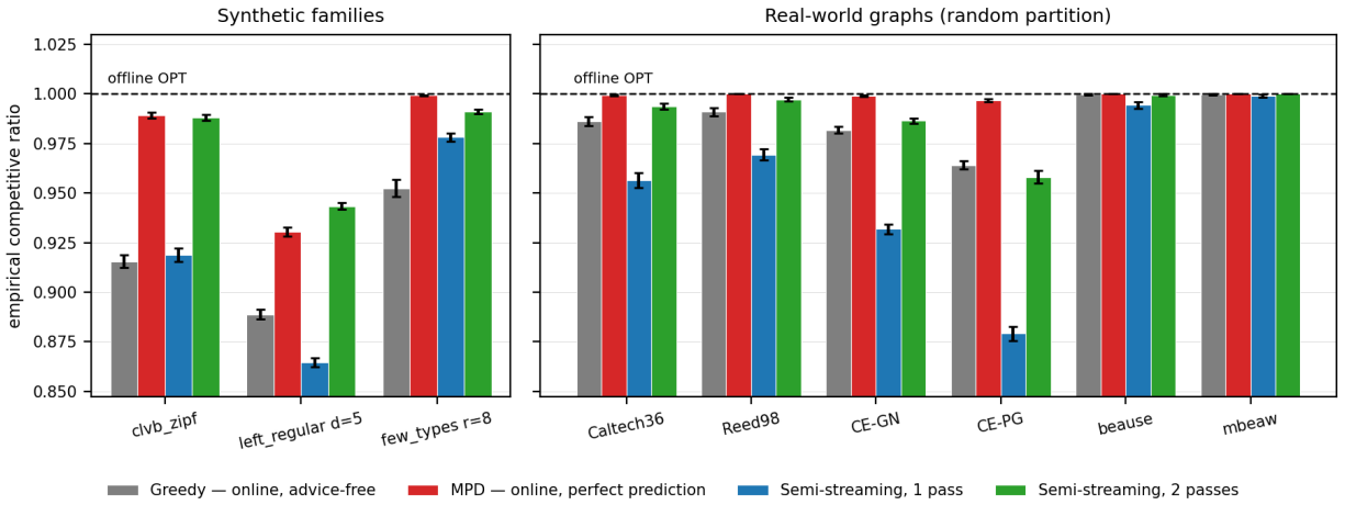
Figure A.1: The relaxation ladder. Grey and red are the online model (advice-free Greedy, and MPD given a perfect degree prediction); blue and green are semi-streaming at one and two passes. On seven of the nine graphs one extra pass buys more than a perfect prediction does.
