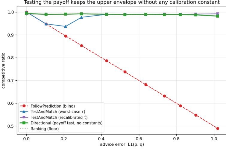
The envelope sweep with the payoff rule added: the worst-case threshold follows the crash at mildly bad advice, the recalibrated threshold never captures at perfect advice, and the constant-free payoff rule tracks the upper envelope within the resolution the budget–stakes law allows.
