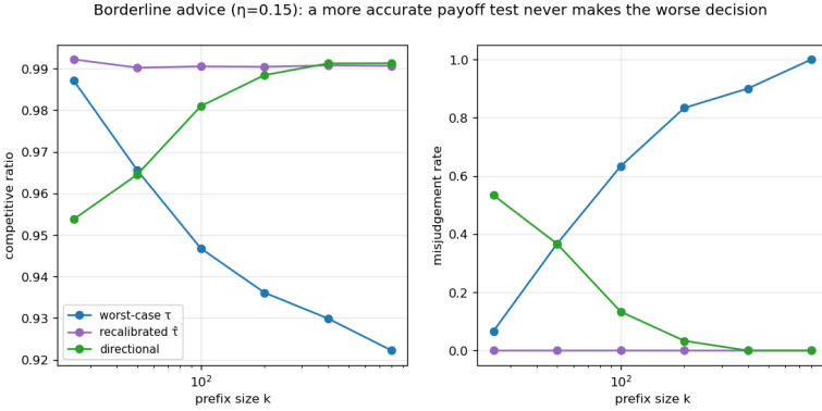
Borderline advice ( \eta = 0.15 ): as the prefix grows, the worst-case threshold’s misjudgement rises to 1.0 while the payoff rule’s falls to 0.0 — more data helps exactly when the statistic is the decision-relevant one.
