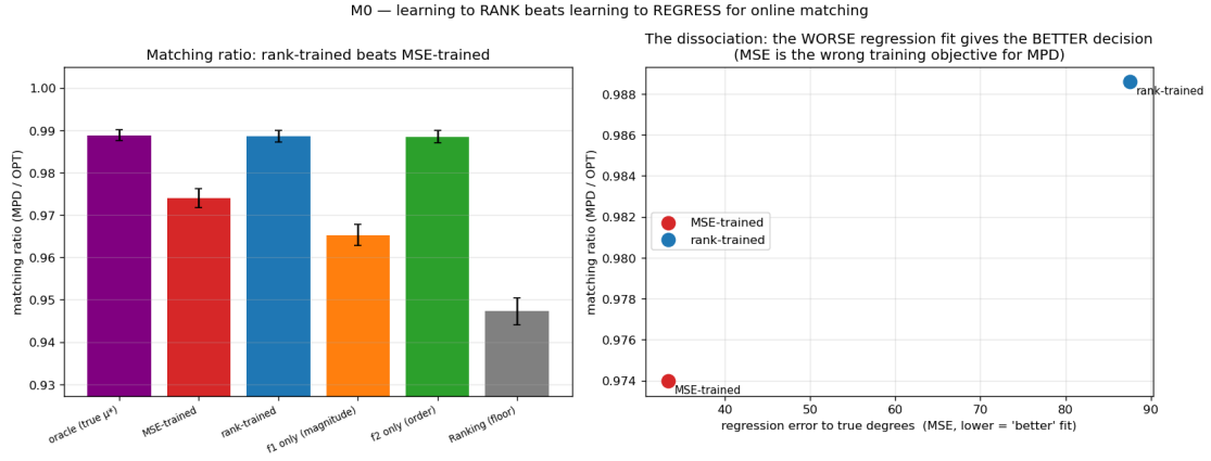
Figure 8.1.: M0: with divergent features, rank-training beats regression on the matching ratio (left) despite a worse regression fit (right).
