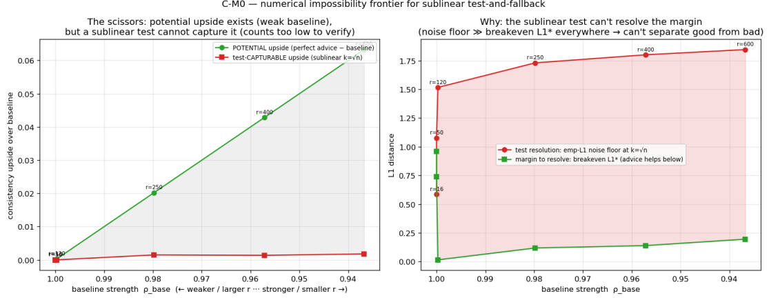
Figure 9.1.: The impossibility scissors: the potential upside grows as the baseline weakens (left), but the upside a sublinear test can safely capture stays near zero; the test’s resolution sits far above the break-even margin (right).
