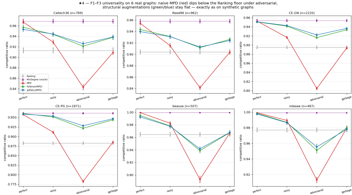
Fig. 8. The six real-world graphs: unguarded following falls below the advice-free floor on every graph, and the augmentation restores safety — the benchmark’s findings are universal, not generator artifacts.
