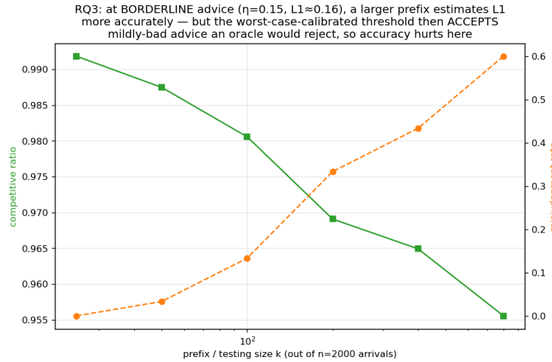
Fig. 4. Testing cost at borderline advice: under the worst-case-calibrated threshold, a larger and more accurate prefix test makes the worse decision.
