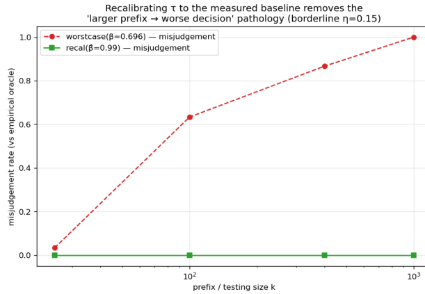
图 3: Recalibration removes the threshold pathology: misjudgement holds at zero at every prefix size, versus climbing toward 1.0 under the worst-case threshold.
