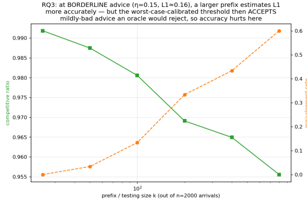
图 2: Testing cost at borderline advice: a larger, more accurate prefix test makes the worse decision under the worst-case-calibrated threshold.
