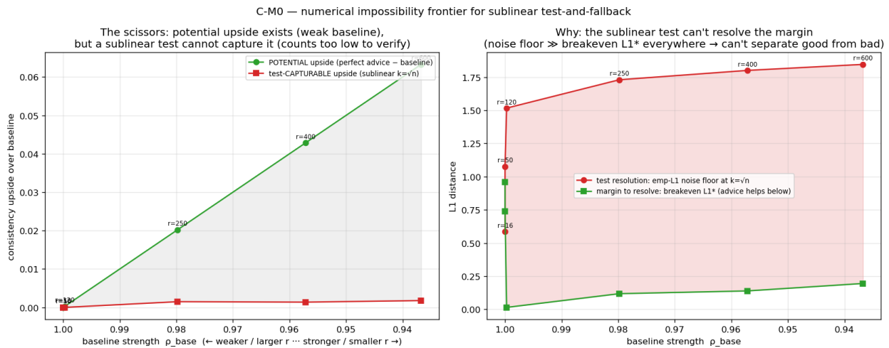
图 4: The testing-wall frontier: as the baseline weakens (left), the potential upside of perfect advice grows, but the upside a sublinear test can safely capture stays near zero —the empirical test's resolution sits far above the break-even margin wherever the upside exists.
