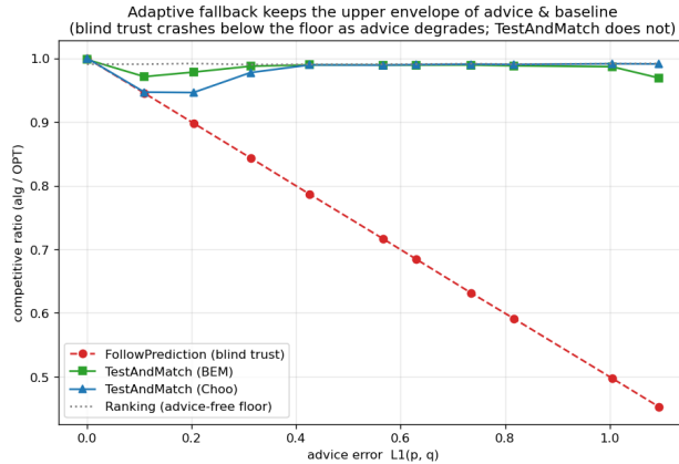
图 1: The robustness envelope: blind FollowPrediction crashes below the advice-free floor as advice error grows; TestAndMatch stays on the upper envelope.
