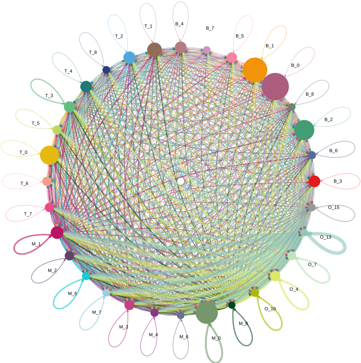
Interaction weights/strength
