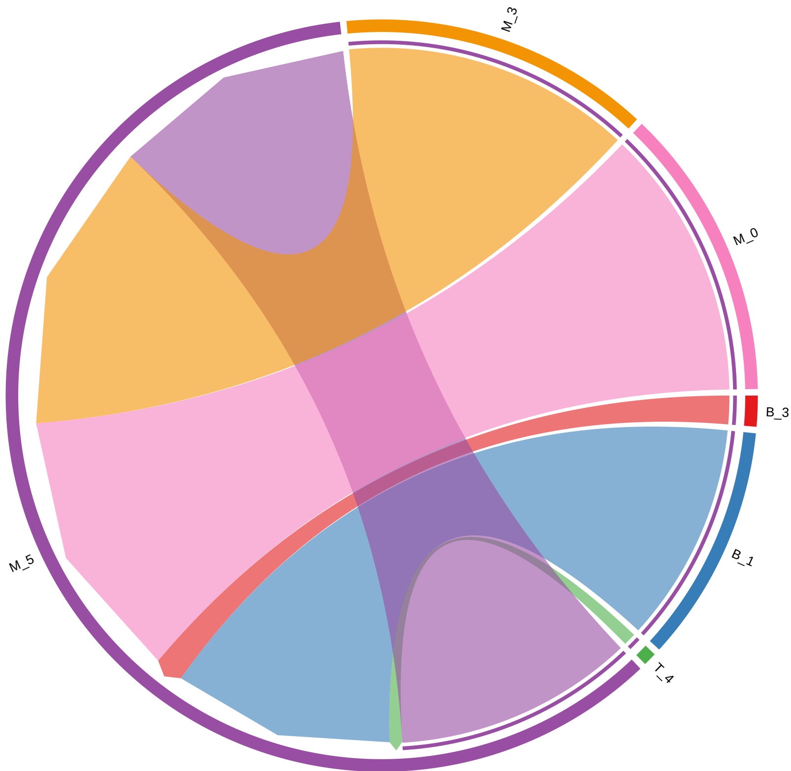
MHC-II signaling pathway network
